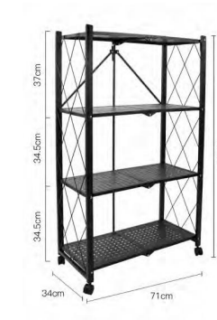
COOE: MH-0680-4 SIZE: 710*390*1250mm
