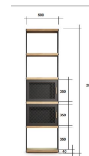
CODE: MH-2037 SIZE: 500*350*2030mm
