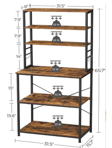
CODE: MH-0569 SIZE: 800*398*1670 mm
